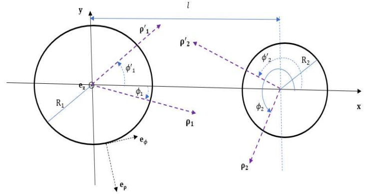
Fig. 2. The coordinate system that defines the system of integral equations (5)
