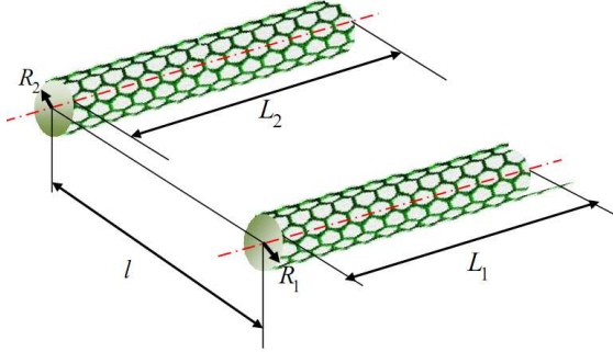
Fig. 1. Configuration of the structure under consideration: A pair of parallel non-identical CNTs with corresponding radii R_{1,2} , lengths L_{1,2} and conductivities \sigma_{1,2} , placed at the distance l one with respect to another.
