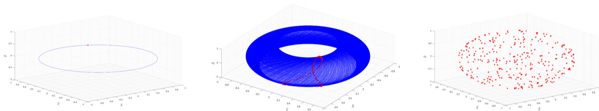
Fig.4: Poincaré maps overlaid on the lab frame physical state space ( Z(X,Y) ) of periodic (left) and quasiperiodic (center) solutions. Poincaré map of a chaotic solution (right).
